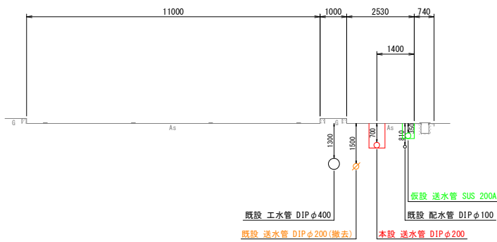
④ — ④' NO. 3
