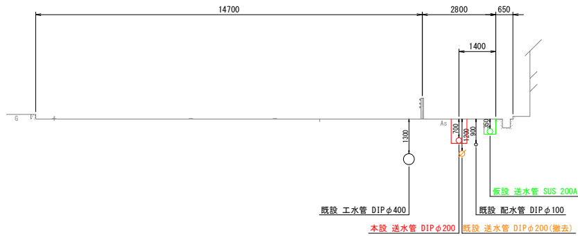
② — ②' NO. 1
