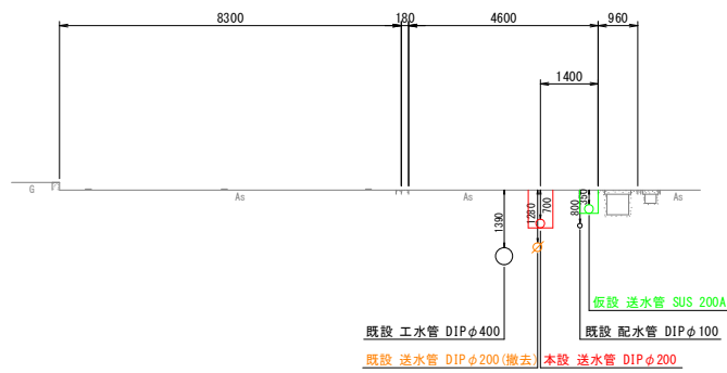
⑦ — ⑦' NO. 7
