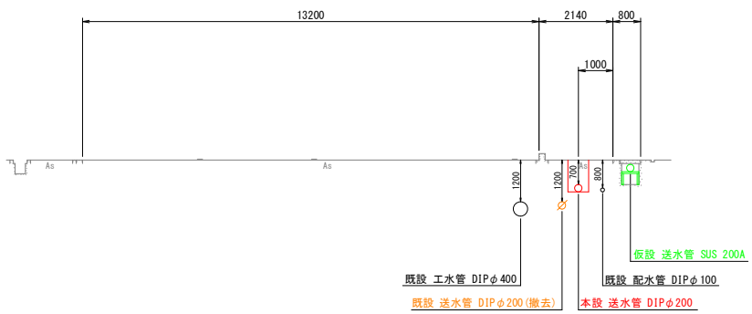
⑩ — ⑩' NO. 10
