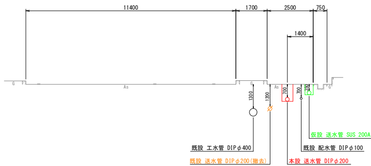
③ — ③' NO. 2
