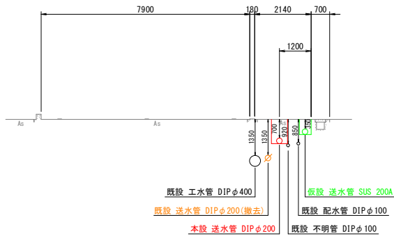
⑩ — ⑩' NO. 10
